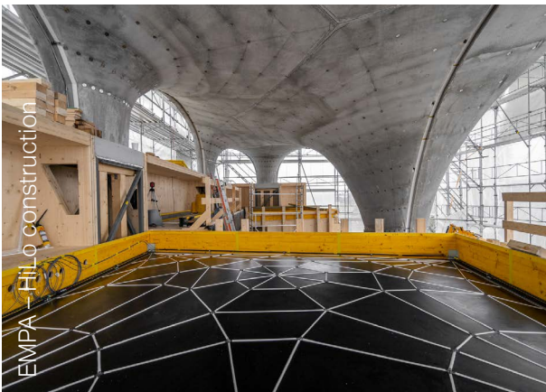
Figure 57: EMPA-ETH Zurich HiLo vaulted flooring system
