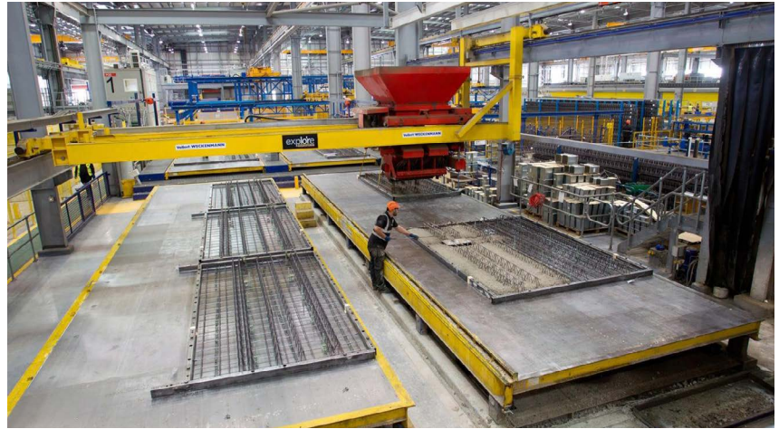
Figure 27: Laing O'Rourke Explore Plant robotically manufacturing precision reinforced concrete building units.
