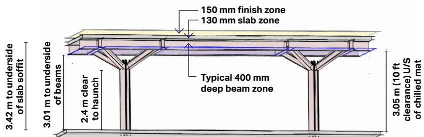
Figure 48: Tree column floor system developed by Make Architects and Arup – effectively shortening the span
