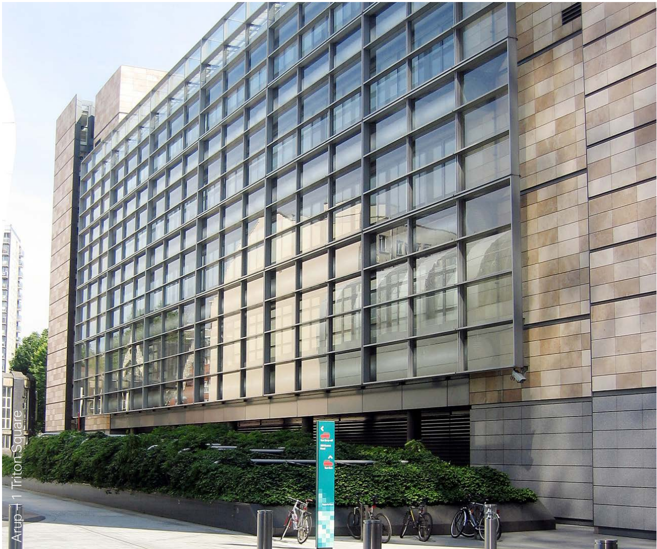
Figure 70: Triton Square, London – 3,000m 2 of façade taken down and refurbished locally to improved performance criteria
