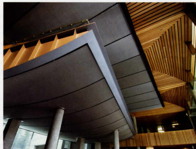
9. The 16m square mezzanine connects to the concrete columns through steel collars and dowels.
