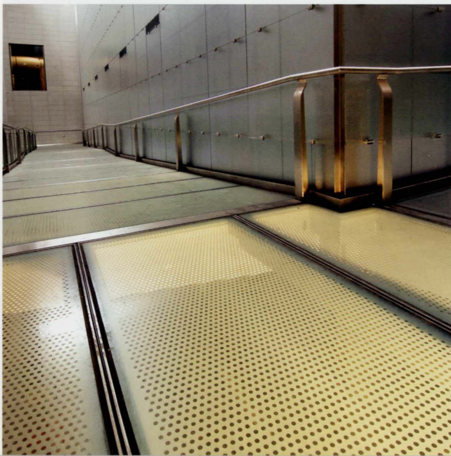
3. The dramatic entry to the new exhibition spaces, showing the steel ramps with glass floor, cantilevered from the side of the exhibition boxes, escalators and circulation spine.
