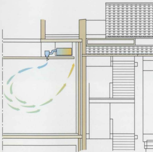
11. Air distribution in temporary exhibition gallery.
