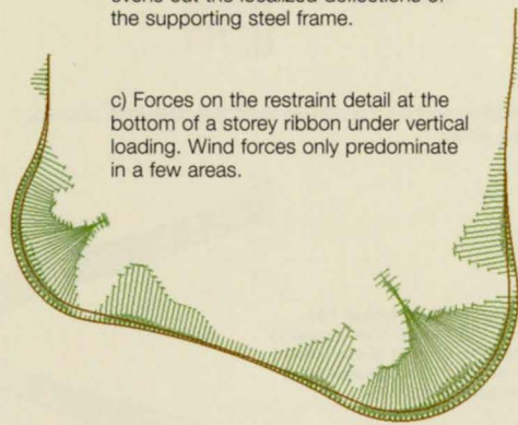
12. GSA analysis of façade.
