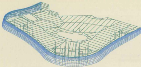
a) Combined floor frame/façade model used to study the composite behaviour of the system.
