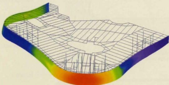
b) Façade displacements around a typical storey ribbon under full loading, showing the extent to which the façade evens out the localized deflections of the supporting steel frame.
