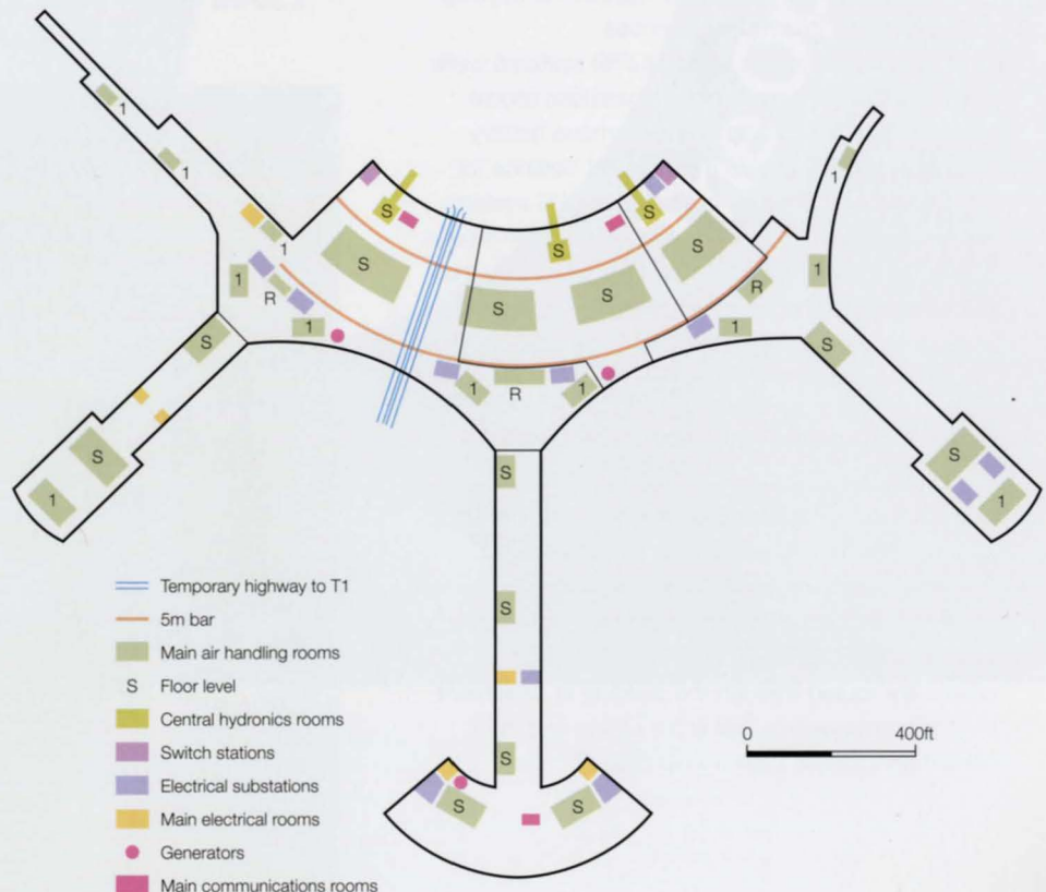
11. Schematic arrangement of primary equipment rooms and risers.
