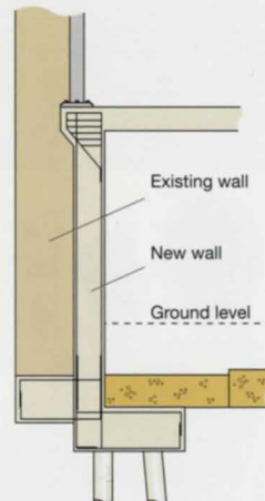
5. Underpinning of existing walls.
