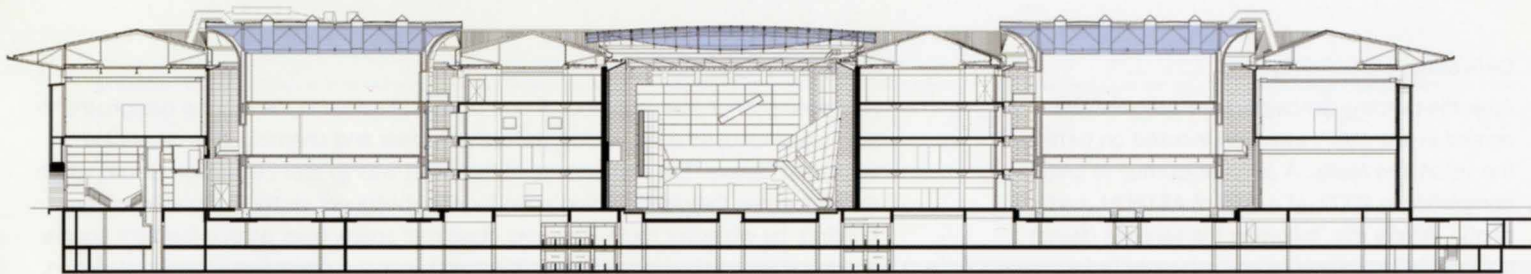
2. Longitudinal section showing, left to right, Coles Court, Federation Court, and Murdoch Court.
