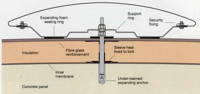
14. Indicative detail of façade construction and fixing.
