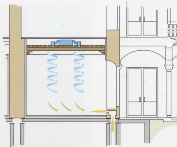
12. Air distribution in permanent gallery.
