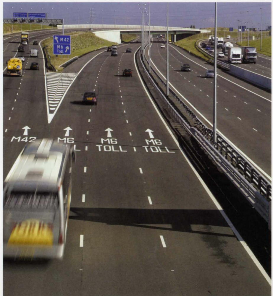
10. M42/M6 Toll junction, where the total width increases to 12 lanes.
