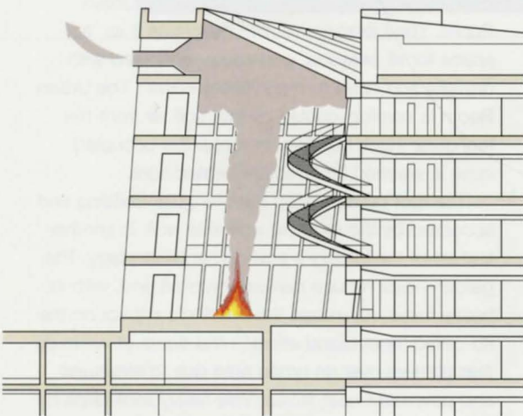
10. Smoke extract strategies for the atria saved costs significantly.
