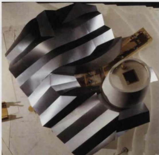
2. Architect's model showing configuration of folded plate roof.
