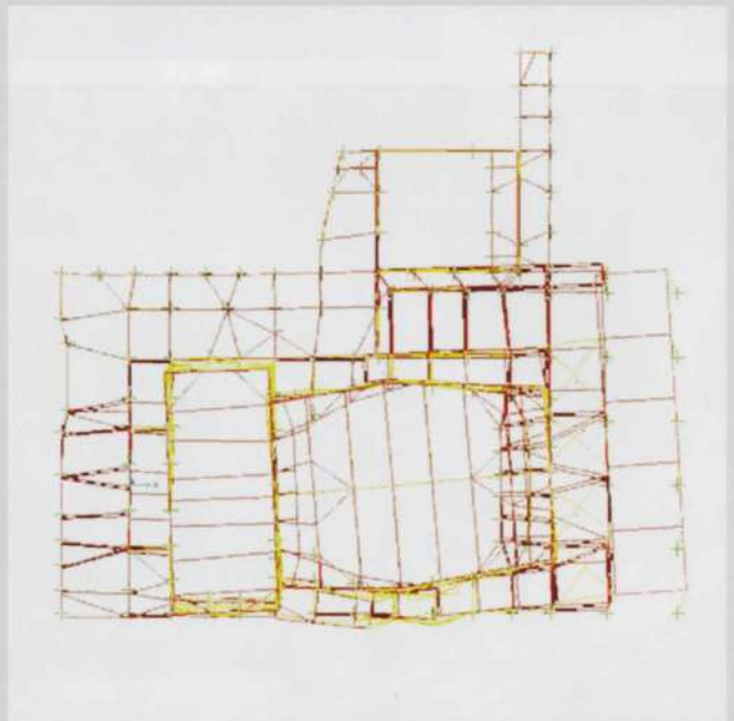
8. Plan view - Mode 3 deflected shape with mass accelerating transversely with torsion.
