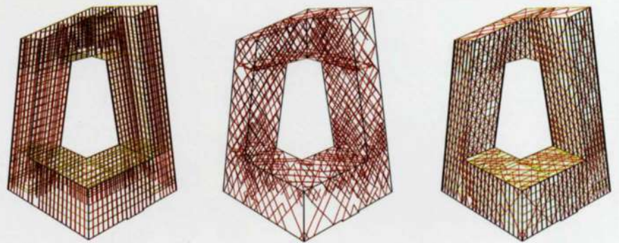
4. Principles of the tube structure: regular grid of columns and edge beams + patterned diagonal bracing = braced tube system.
