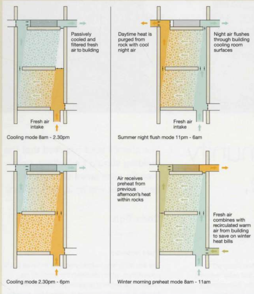
11. Rockstore operation modes.
