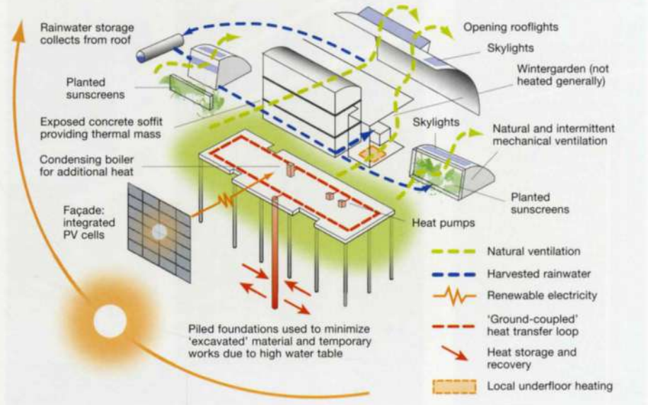
2. Energy-saving structural and services concepts.
