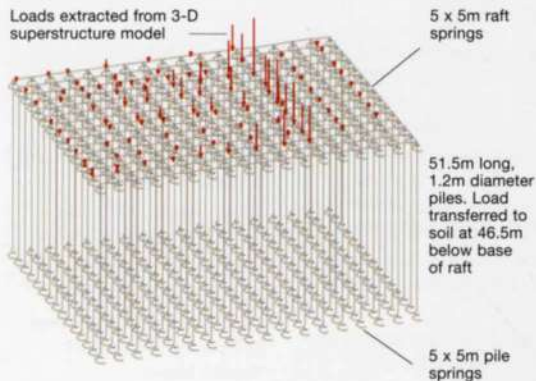
11. GSraft model of the piled foundation.
