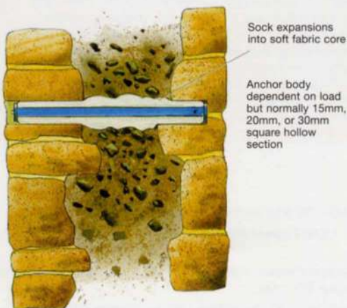
23. Wall stitching with grouted anchors: length, number, and position dependent on structural condition.
