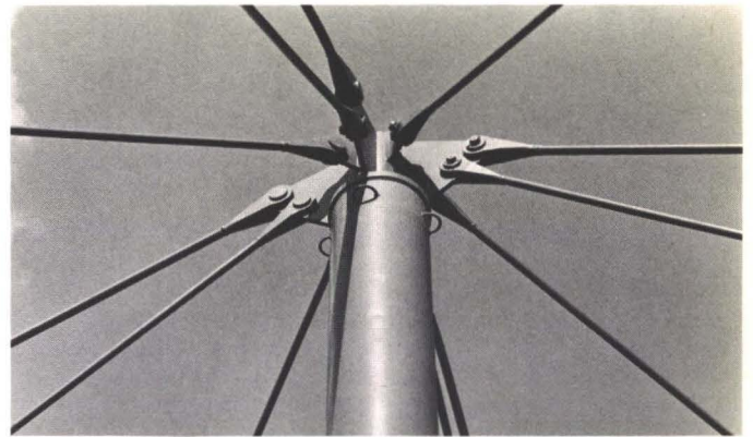
Fig. 13 Boom end detail
