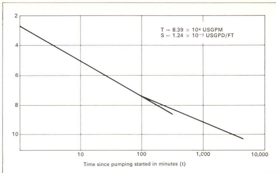
Fig. 11 Time drawdown curve for observation borehole 'A'
