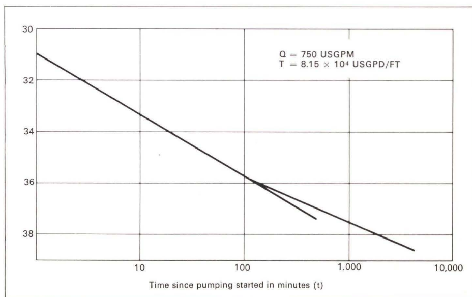
Fig. 12 Time drawdown curve for production borehole 'B'
