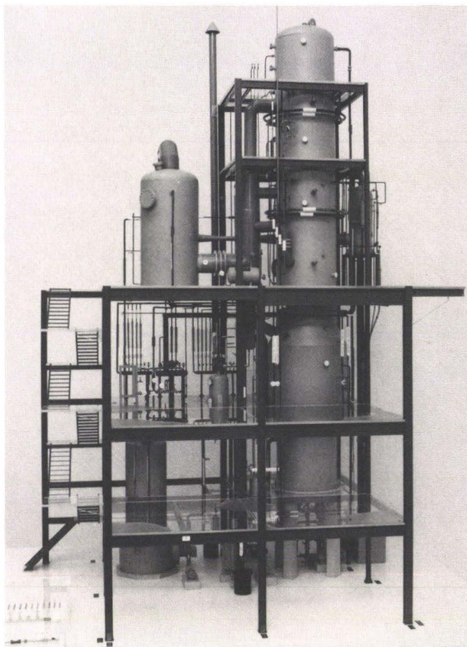
Fig. 14. Model of Lever Brothers refinery (Photo : Unilever, London)
