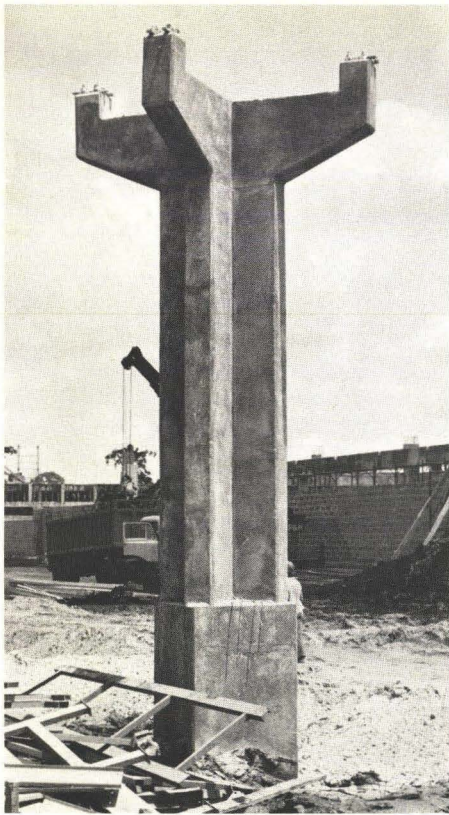
Fig. 16 Cruciform column to carry pipe bridge (Photo: Bill Haigh)
