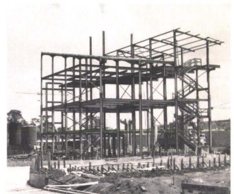
Fig. 15 Erection of refinery steelwork (Photo : Bill Haigh)
