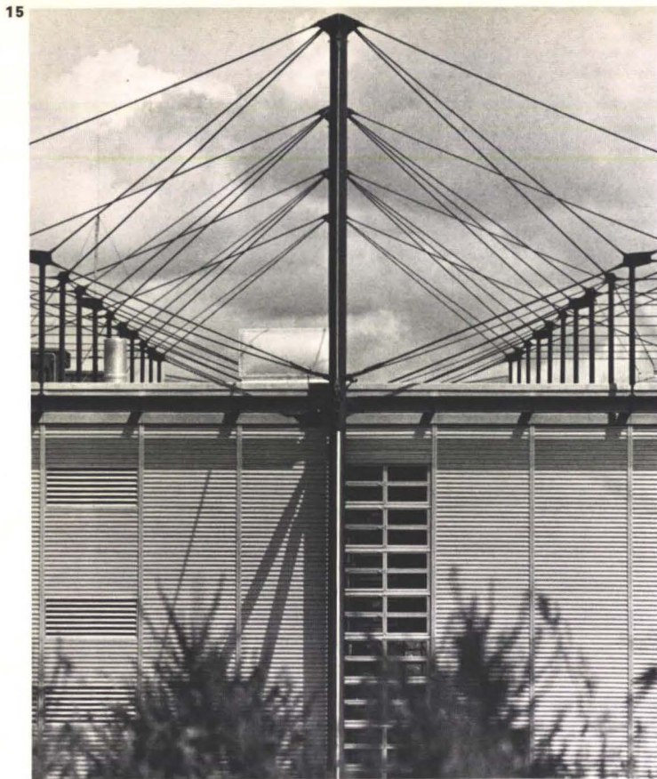
Fig. 15 Detail of elevation showing one of the many patterns of symmetry of the rods
