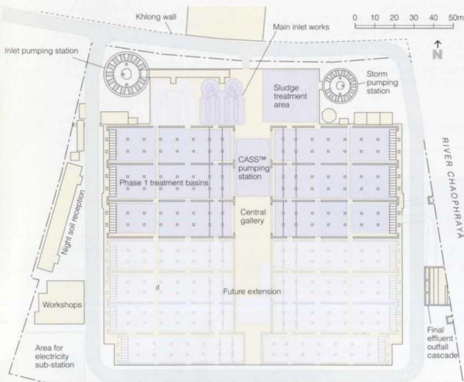
7. Plan of wastewater treatment plant.
