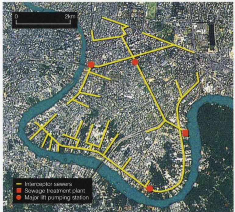
1. The Yannawa Project area in central Bangkok.
