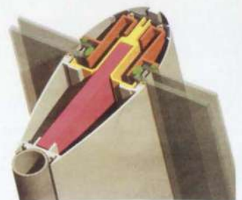
4. 3D rendering of aluminium glazing mullion.
