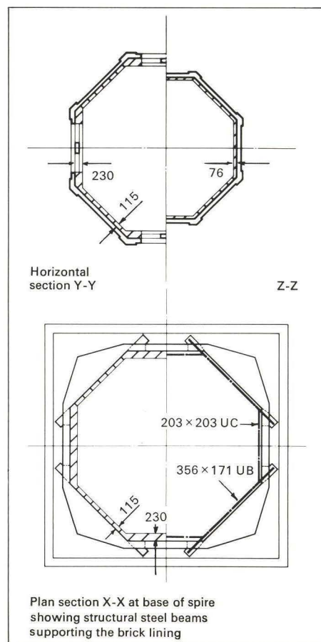
Fig. 13 Horizontal sections through tower and brick lining
