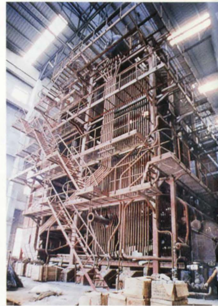
9. Boiler under construction in the Energy Centre.
