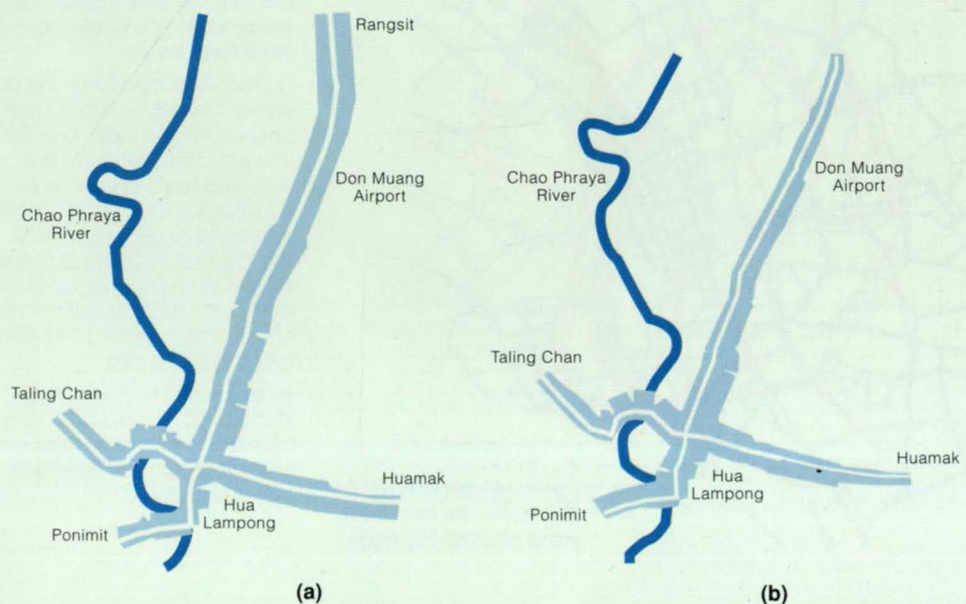
5. Forecast demands for BERTS; (a) tollway (bandwidth indicates scheme loading in am peak period); (b) CT system (bandwidth indicates scheme patronage in am peak period).
