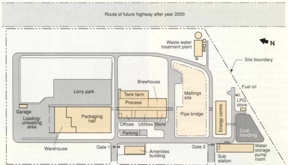
3. Layout of Baoding Brewery.
