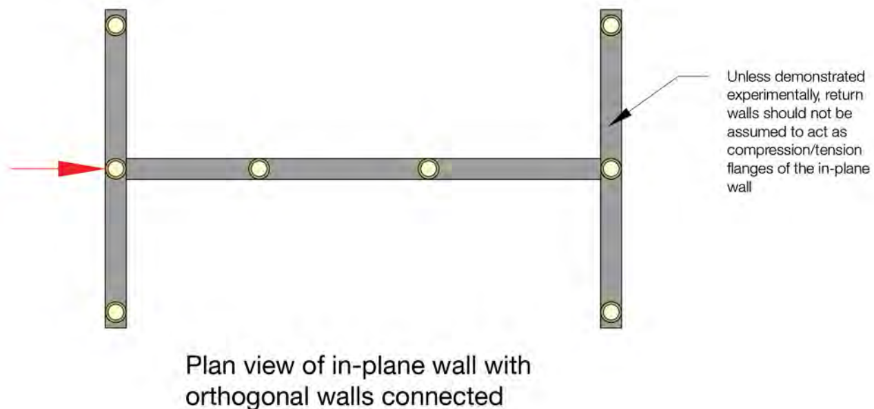
Figure 8.14: Limitations on composite action of CBSW with flanges of return wall when in flexure
