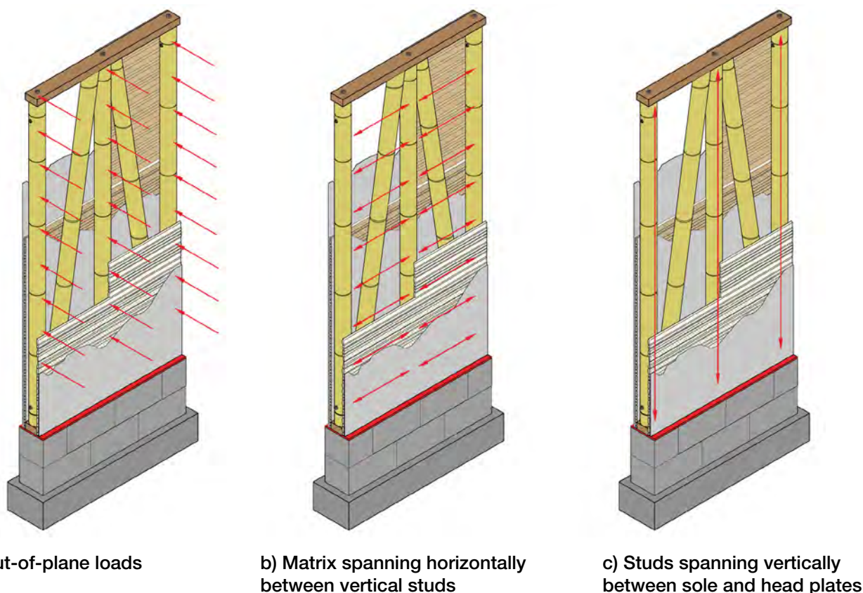
Figure 8.11: Out-of-plane load path for CBSW panels
