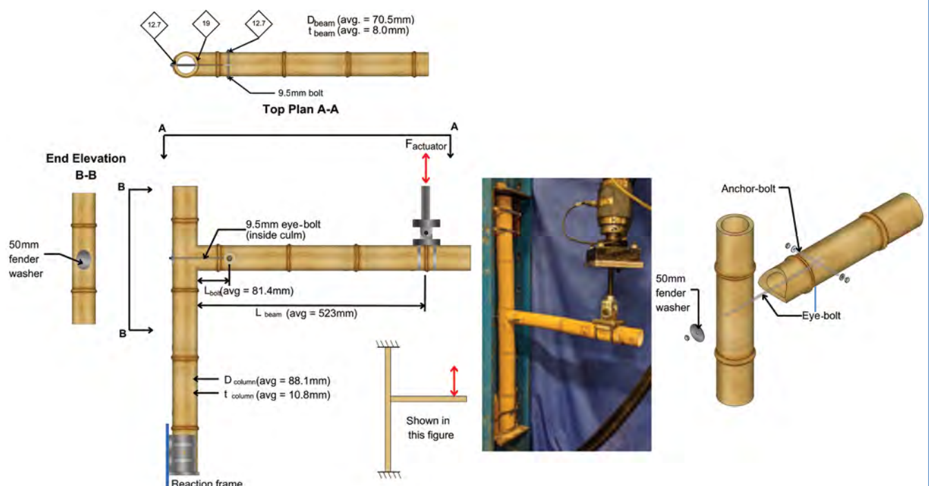
Figure 10.6: Test arrangement and details of T-shaped connection
