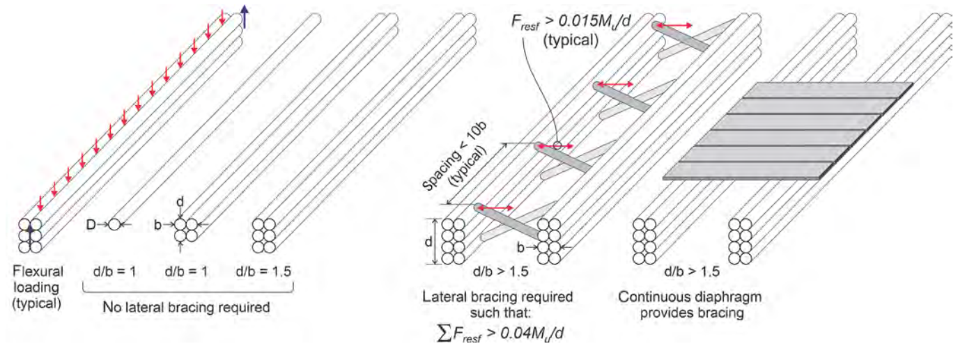
Figure 6.8: Lateral bracing requirements
