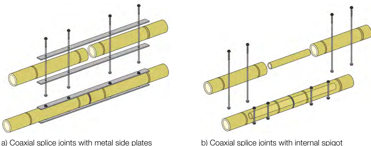
Figure 7.5: Splice joints
