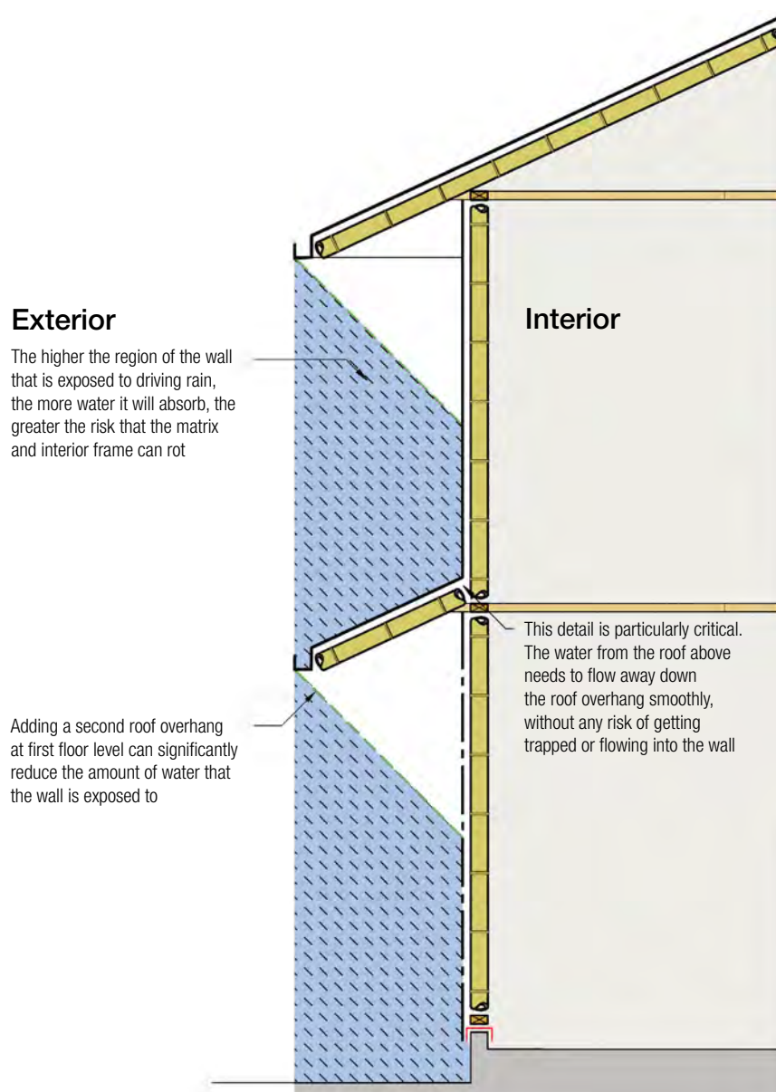
Figure 8.6: Additional considerations for two-storey housing
