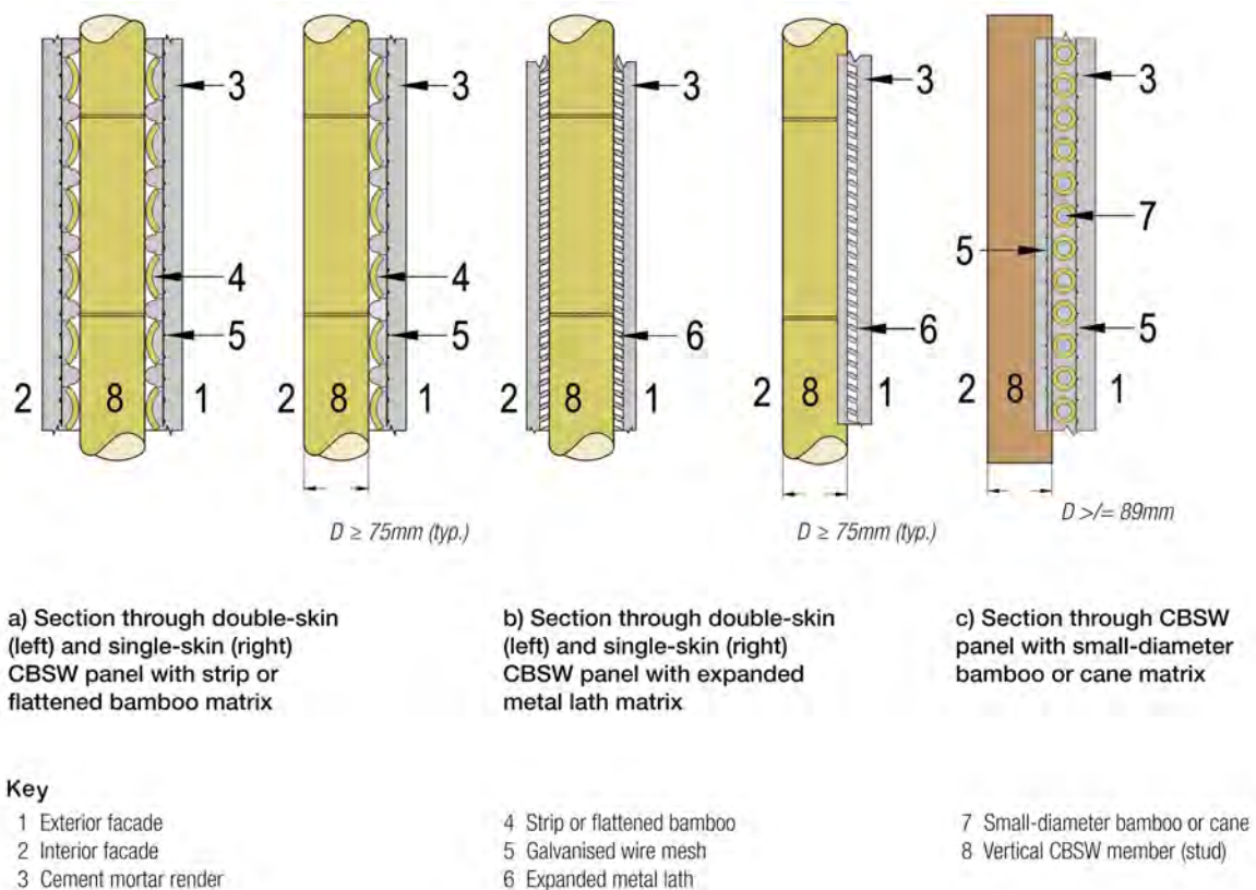
Figure A8.2: Typical sections through CBSW panels with different matrices
