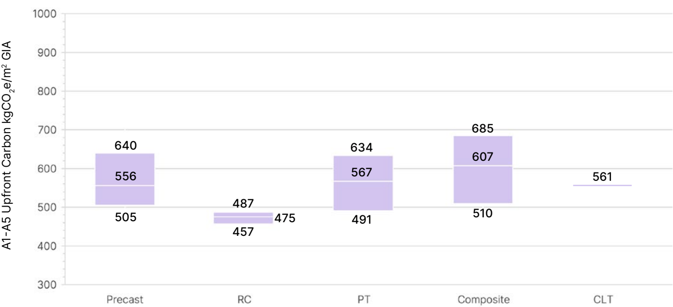
S&C Upfront Carbon vs Structural Floor Systems
