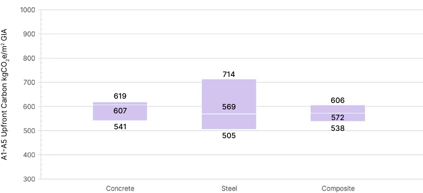
S&C Upfront Carbon vs Structural Frame Systems
